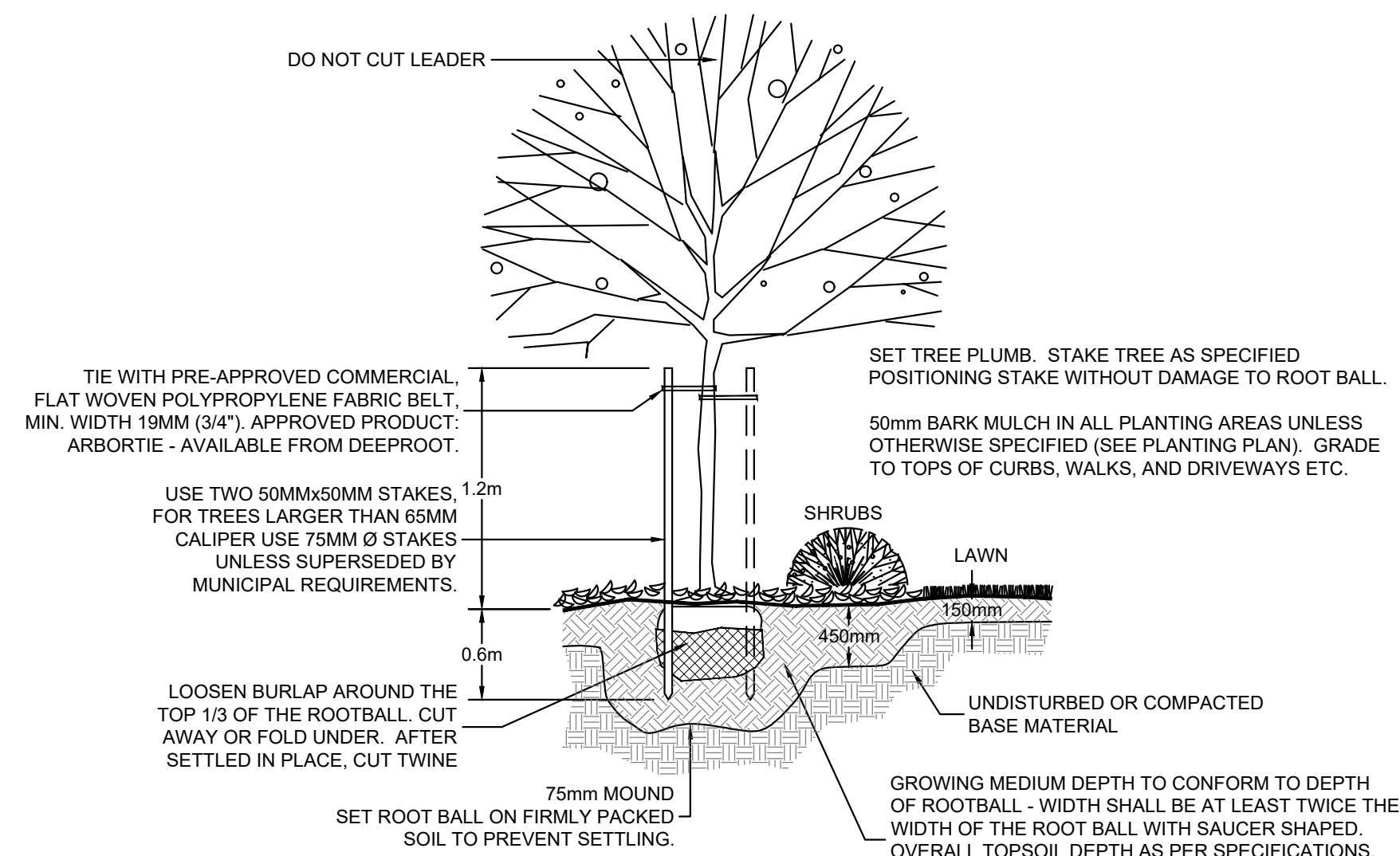
7 TREE/SHRUB PLANTING DETAIL 1:25
