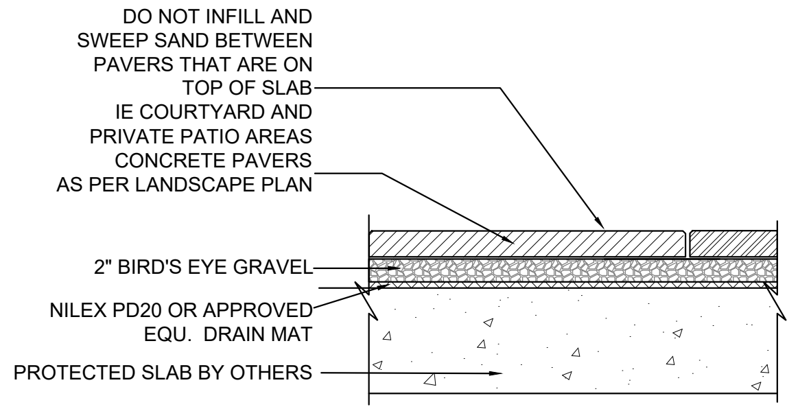
3 PAVERS ON SLAB 1:10
