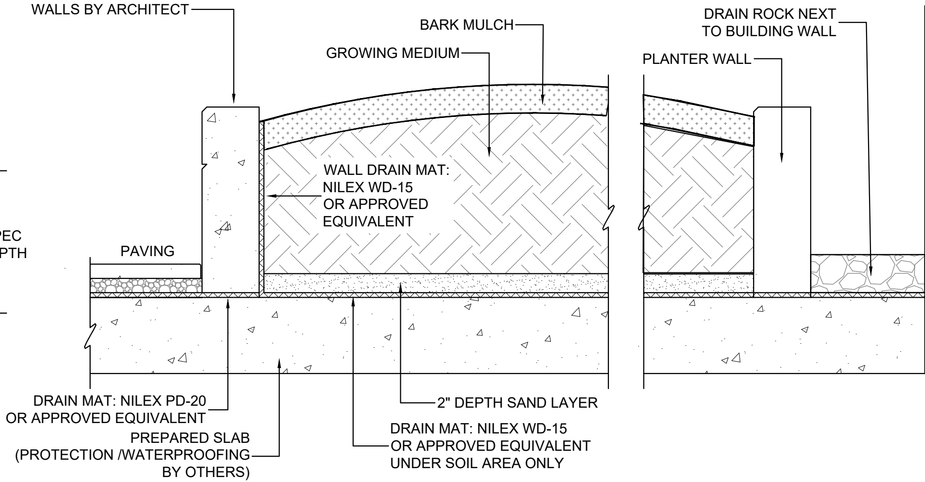
2 PLANTER WALL ON SLAB 1:10
