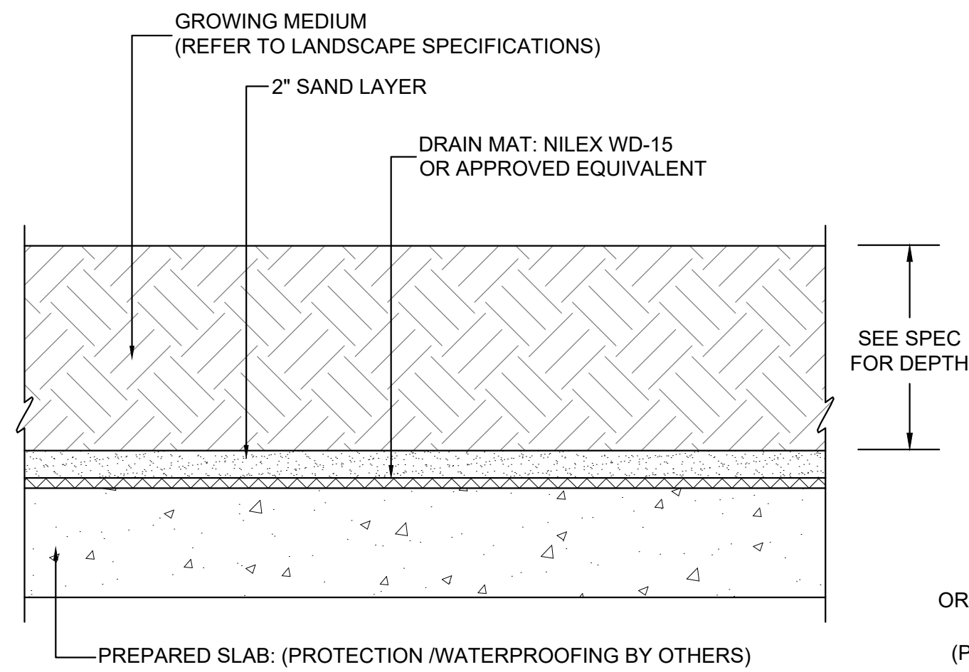
1 PLANTING ON SLAB 1:10
