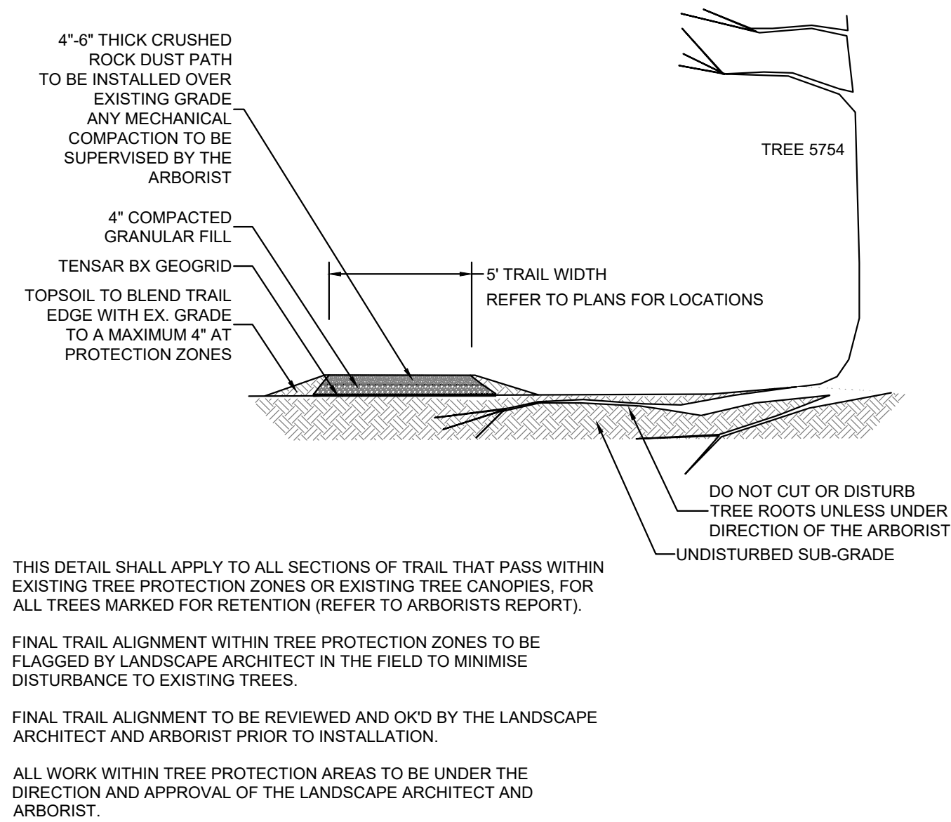
5 5' CRUSHED ROCK DUST PATH 1:50
