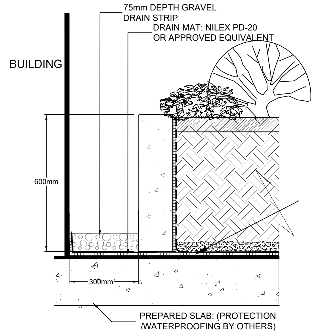
4 DRAIN STRIP ON SLAB 1:10
