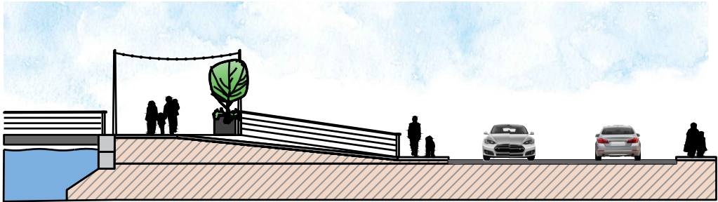
LANDSCAPE CONCEPT SECTION B - B'
